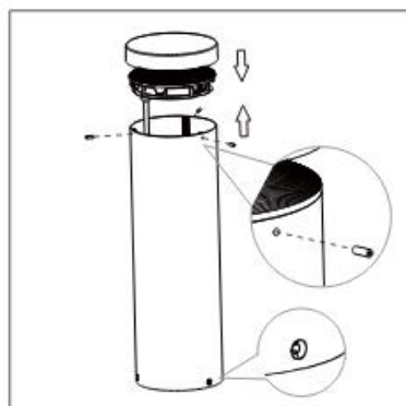
7. Fix the bollard head and bollard tube
